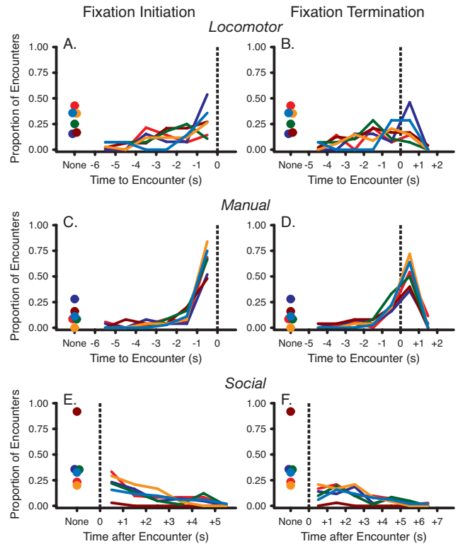
Figure 5 Individual histograms for the initiation and termination times for each of the 6 infants' fixations for locomotor, manual, and social encounters. "None" refers to the proportion of encounters that infants did not fixate the target. Vertical dashed lines indicate the moment that defined each encounter.
